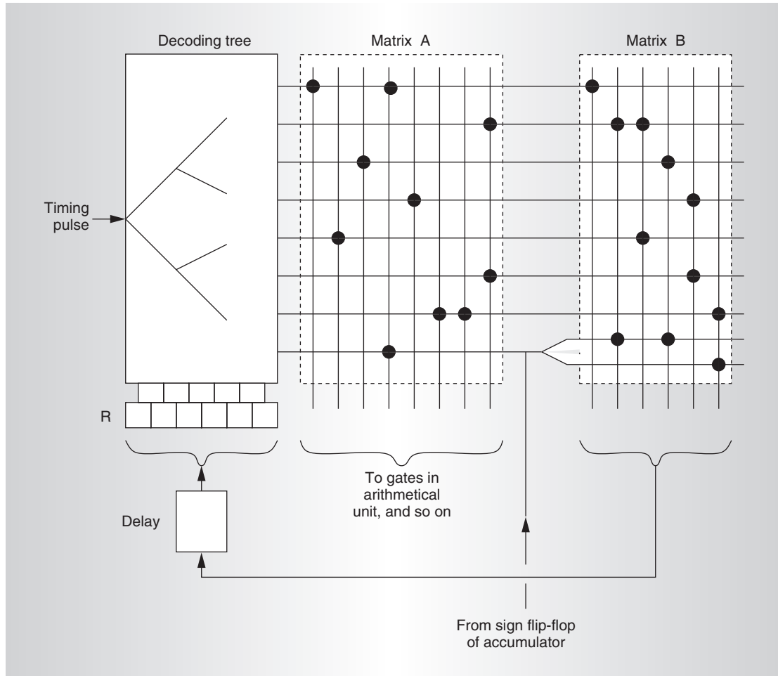
Figure 1. Wilkes' microprogram control model.
