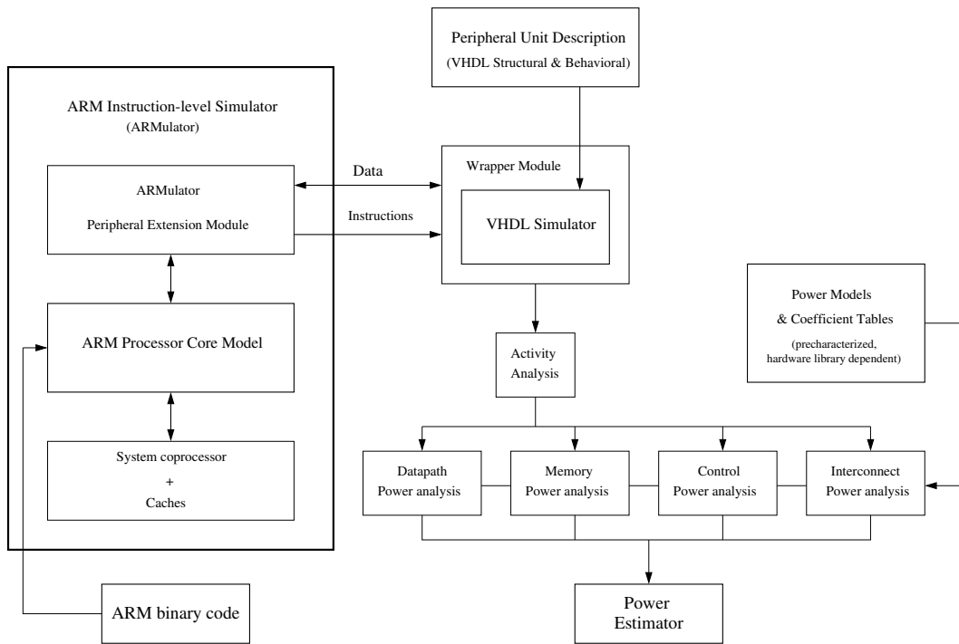
Fig. 1. System-on-chip simulator architecture.
