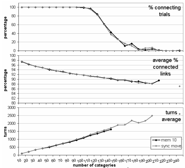
Figure 3: memory interval [1, 10]; sequential vs. synchronous cluster movement
