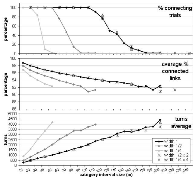
Figure 5: ‘triangular’ matching functions with varying widths
