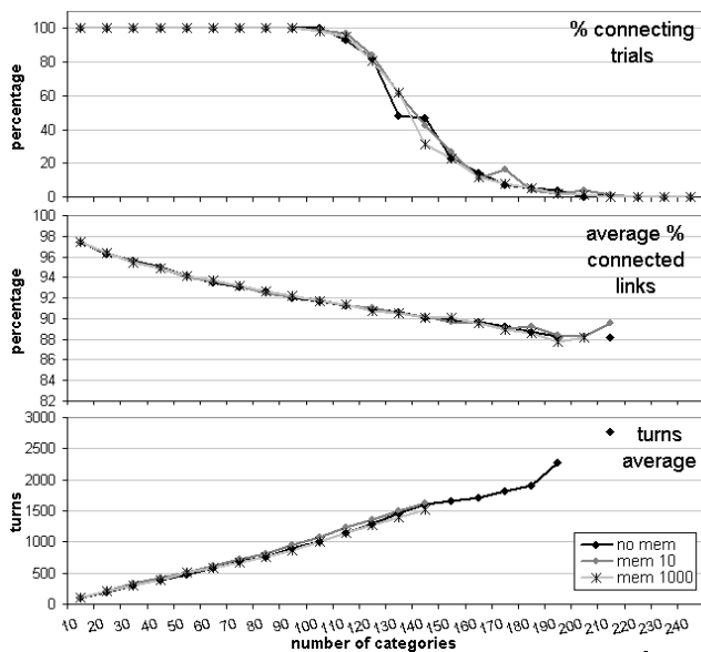
Figure 2: no memory v.s. memory of intervals [1,10] and [1,1000]
