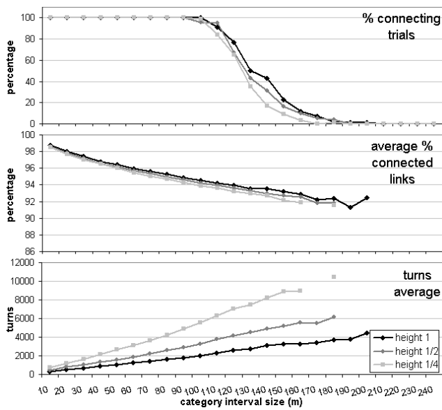
Figure 6: ‘triangular’ matching functions with varying heights
