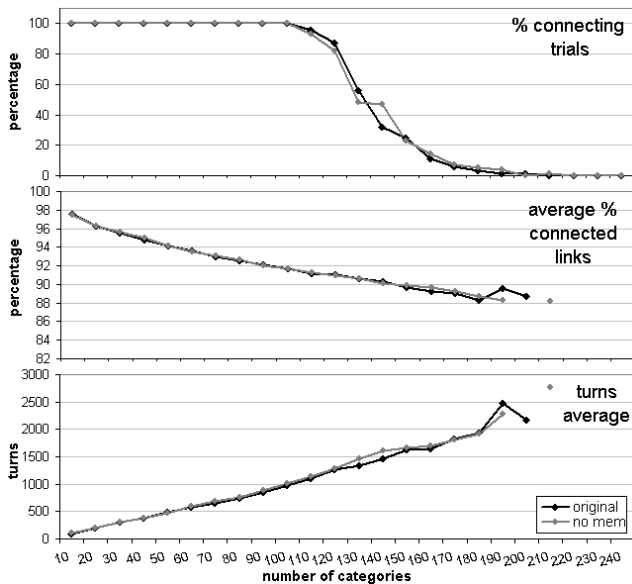
Figure 1: original synchronized system vs. no memory unsynchronized system
