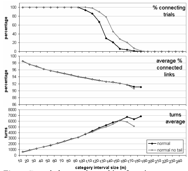
Figure 7: scaled normal matching function vs. same cut off at 1/2
