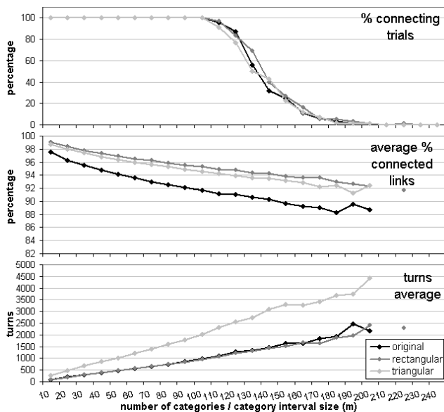
Figure 4: original discreet system compared to a continuous systems with ‘rectangular’ and ‘triangular’ matching functions
