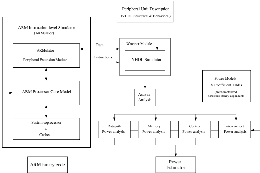
Fig. 1. System-on-chip simulator architecture.
