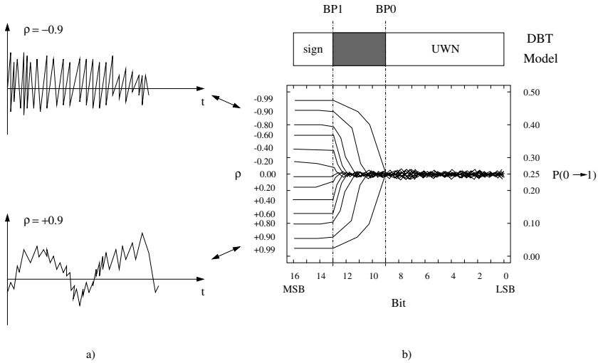
Fig. 2. Bit transition activity for 2 two’s complement data streams modeled as Gaussian processes with different temporal correlation \rho : a) Activity for positively and negatively correlated waveforms. b) Bit transition activity for data streams with varying temporal correlation.
